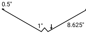
W-Valley
