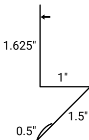
Rat Guard
