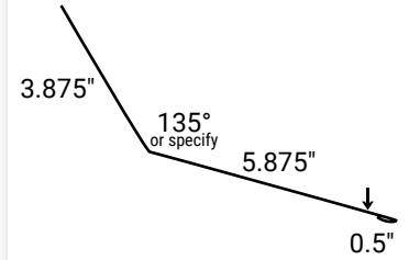
Endwall/Pitch Break
