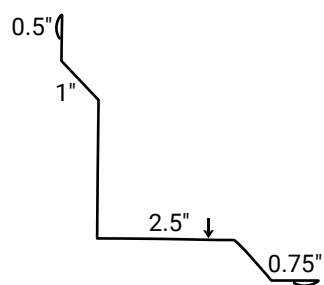
SM Inside Corner
