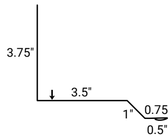
Sidewall
