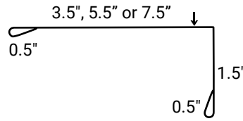
Fascia/Eave (1.5 x 3.5, 5.5 or 7.5)
