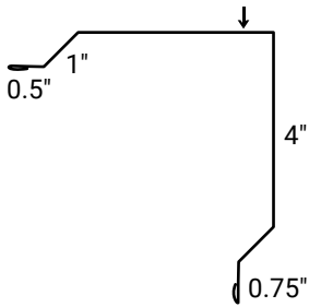
LG Outside Corner
