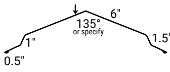
16" Ridge
