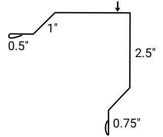
SM Outside Corner
