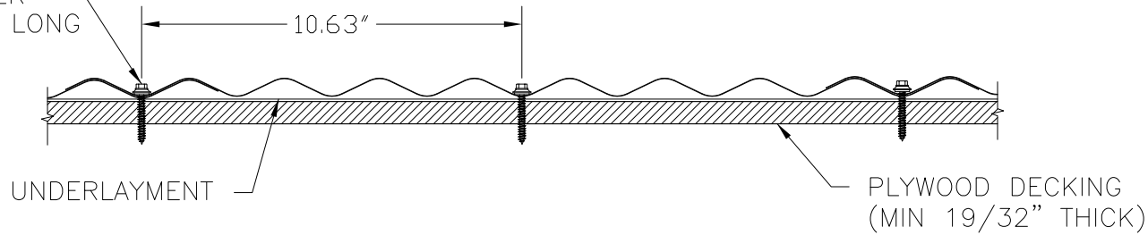
FASTENER PATTERN @ INTERMEDIATE LOCATIONS
