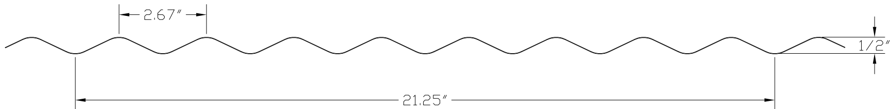
Corrugated Panel Profile
