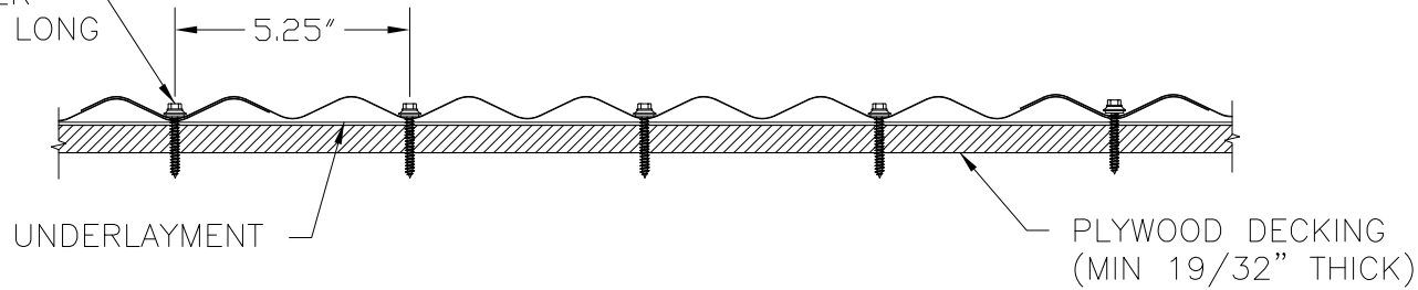
FASTENER PATTERN @ EAVE, RIDGE & VALLEY
